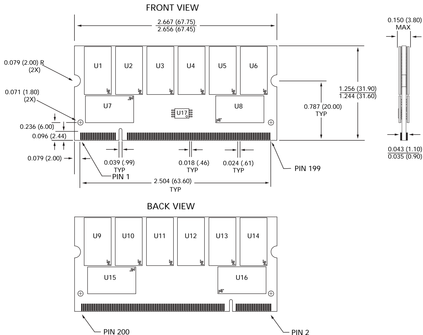
Figure 16: 200-PIN SODIMM Dimensions – 512MB
