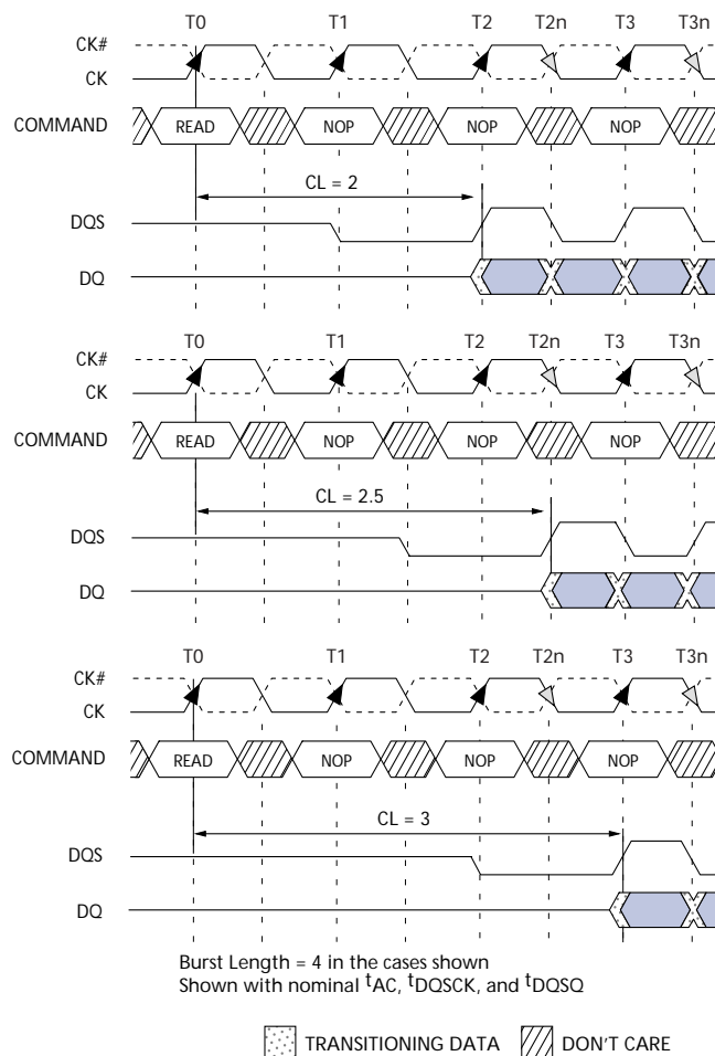
Figure 6: CAS Latency Diagram
