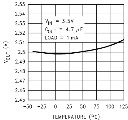
Figure 5-1. V_{OUT} vs Temperature for Legacy Chip
