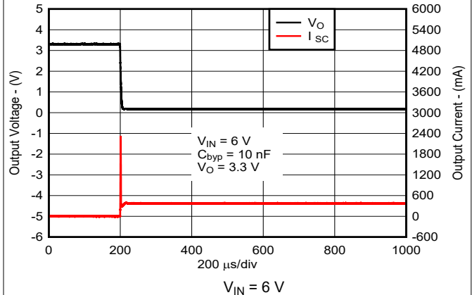
Figure 5-4. Short-Circuit Current vs Time for New Chip
