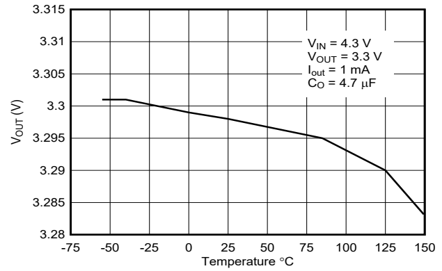
Figure 5-2. V_{OUT} vs Temperature for New Chip
