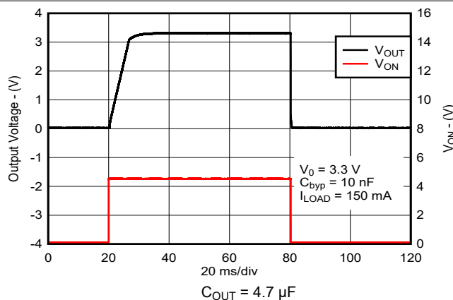
Figure 5-58. Turn-on Time for New Chip
