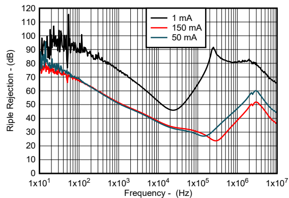
V_{IN} = 3.7 V , V_{OUT} = 3.3 V , C_{OUT} = 10 \mu F , C_{BYP} = 0 nF Figure 5-17. Ripple Rejection vs Frequency for New Chip
