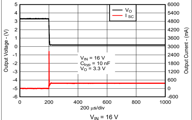
Figure 5-6. Short-Circuit Current vs Time for New Chip
