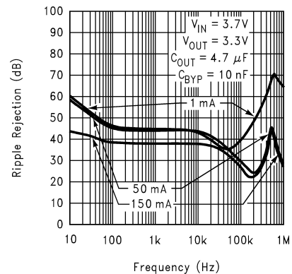
Figure 5-16. Ripple Rejection vs Frequency for Legacy Chip
