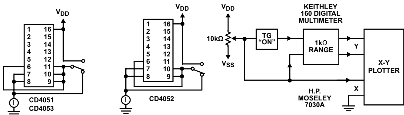
Figure 7-10. Quiescent Device Current
