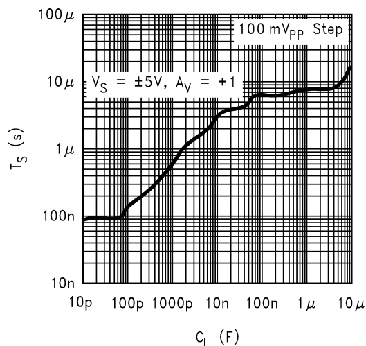
Figure 61. ±5% Settling Time vs. Capacitive Load
