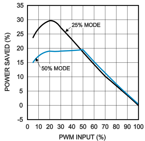
Power saved with PWM & current mode compared to PWM mode
