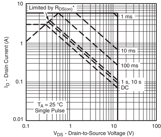
* V_{GS} > \text{minimum } V_{GS} \text{ at which } R_{DS(on)} \text{ is specified} Safe Operating Area, Junction-to-Foot
