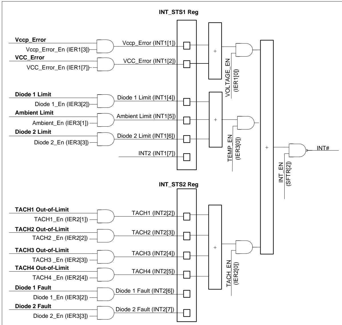
Figure 6.1 Interrupt Control
